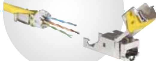
Pass the cable through the back of the wire housing
