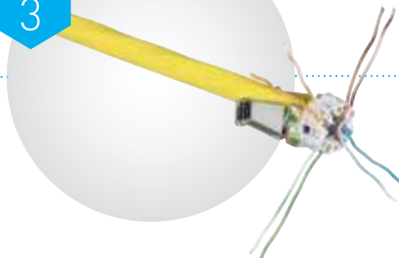
Separate and insert the pairs
